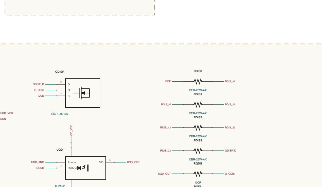
CONTROL / GROUNDING
