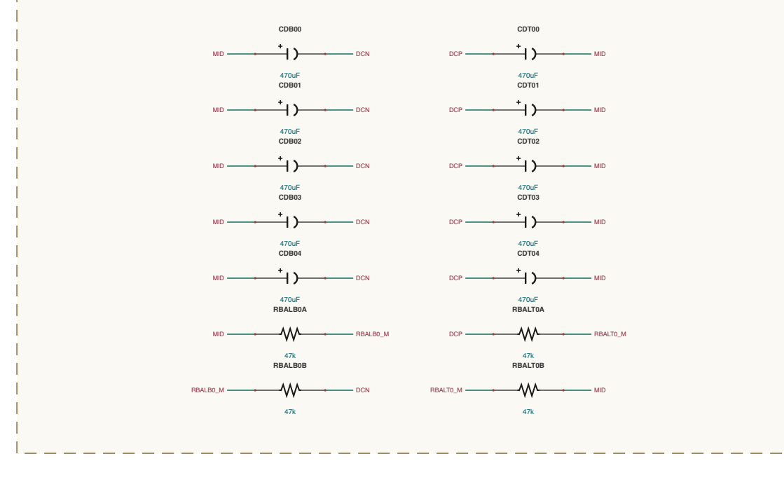
DC-LINK / BUS-STOP
