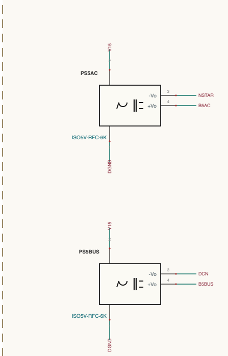
AC-SENSING / ISO-BIAS
