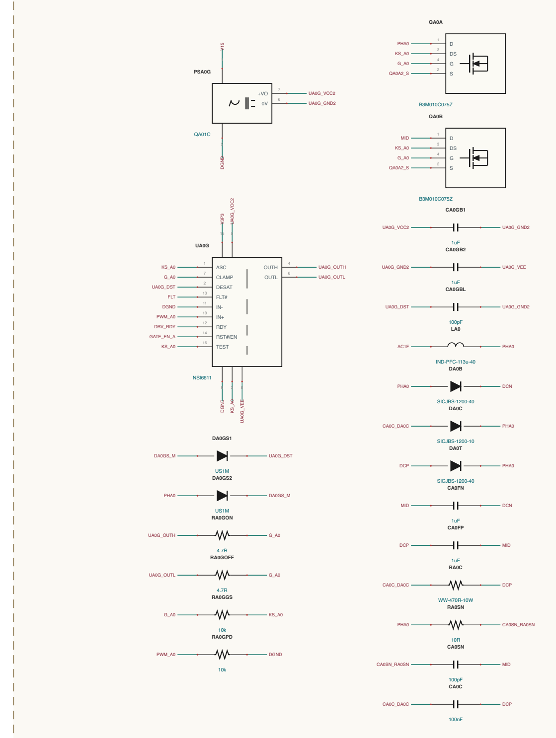
VIENNA-PFC / PHASE-A0
