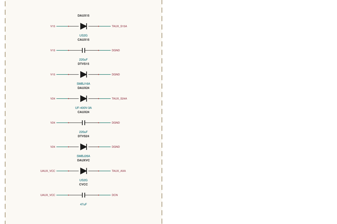
AUX-POWER / RAILS
