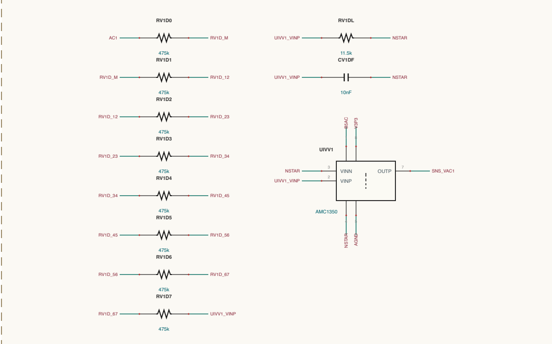
AC-SENSING / SENSE-VAC1
