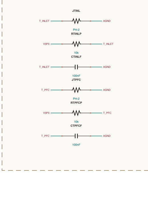
AC-SENSING / NTC
