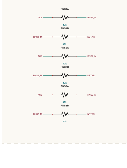
AC-SENSING / STAR
