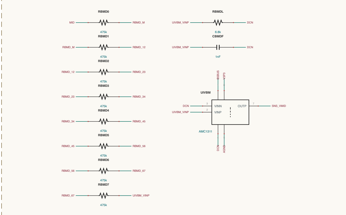
AC-SENSING / SENSE-VIND
