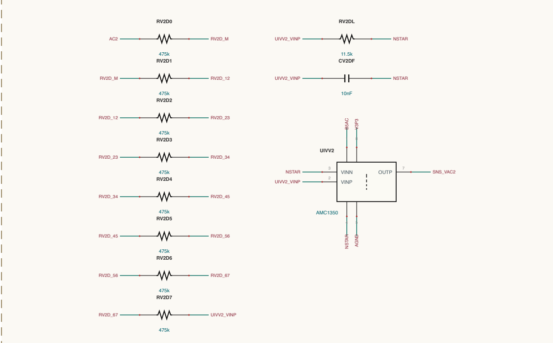
AC-SENSING / SENSE-VAC2
