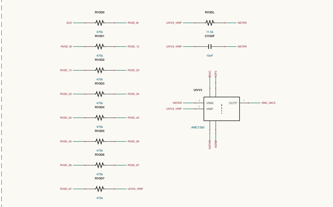
AC-SENSING / SENSE-VAC3
