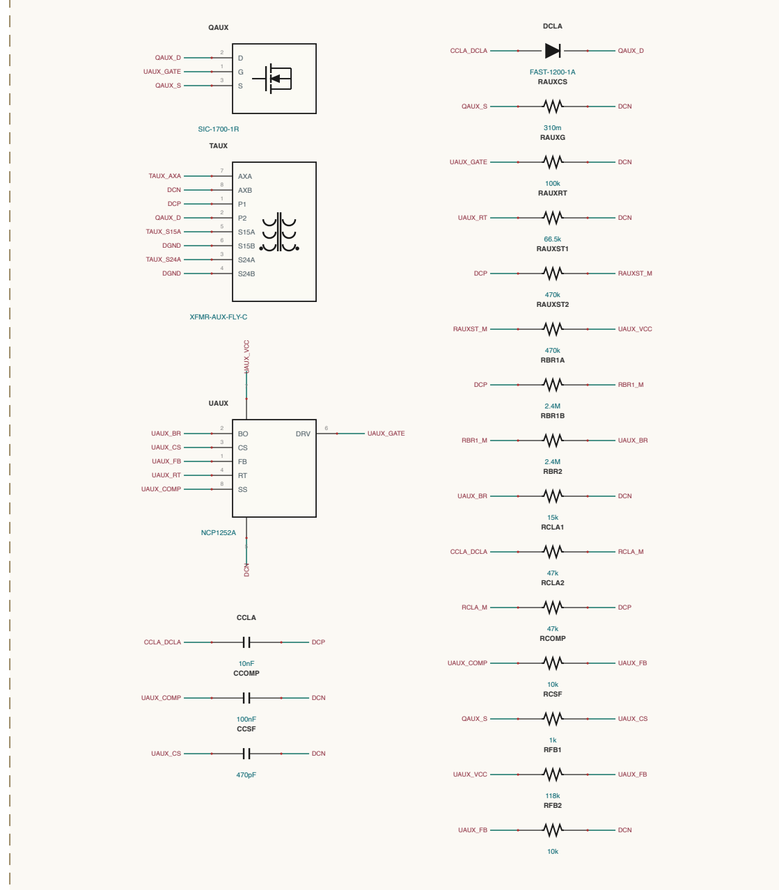
AUX-POWER / FLYBACK
