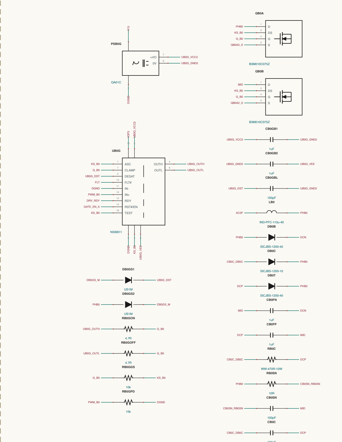
VIENNA-PFC / PHASE-B0
